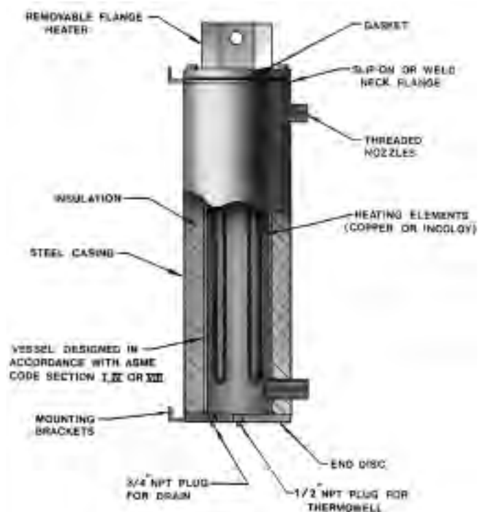
FIG. 2 - CONSTRUCTION DETAILS
