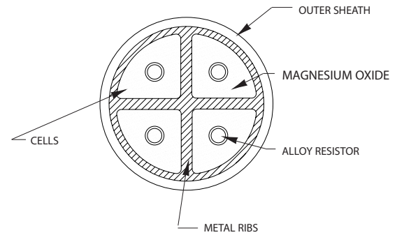
FIGURE 2 - TYPE MH MITOSIS HEATER CROSS SECTION
