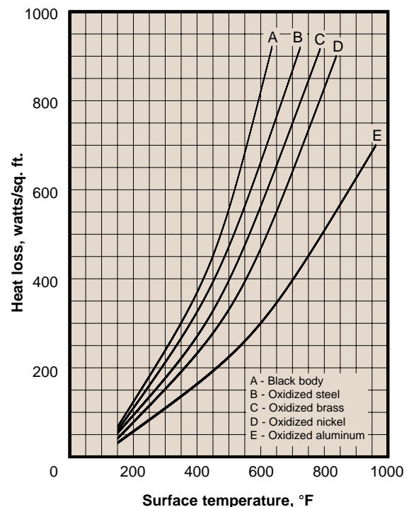
Figure 2 - Heat losses from uninsulated smooth solid surfaces (150 - 1000°F). Assumed external ambient temperature of 70°F.
