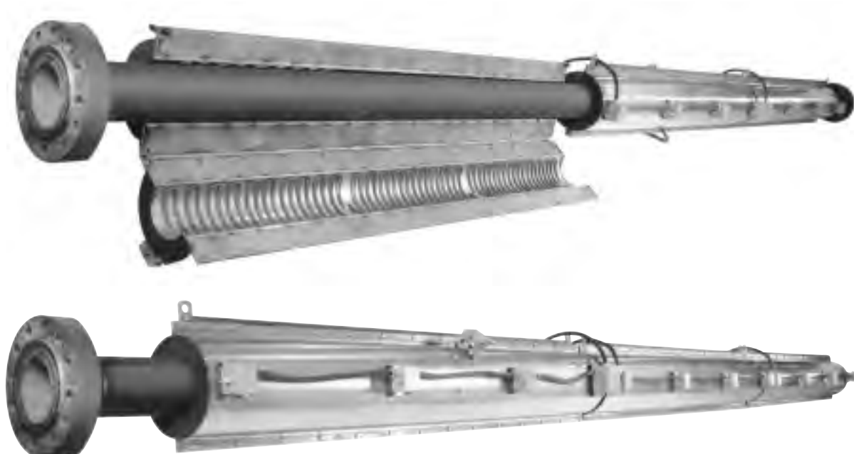
HIGH PRESSURE GAS PREHEATER 480V 3Ø 58KW
