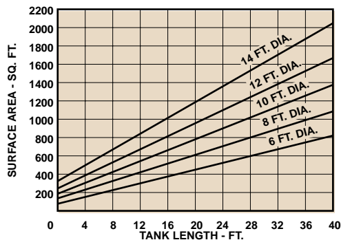
FIG. 2 - TANK SURFACE AREA vs. LENGTH
