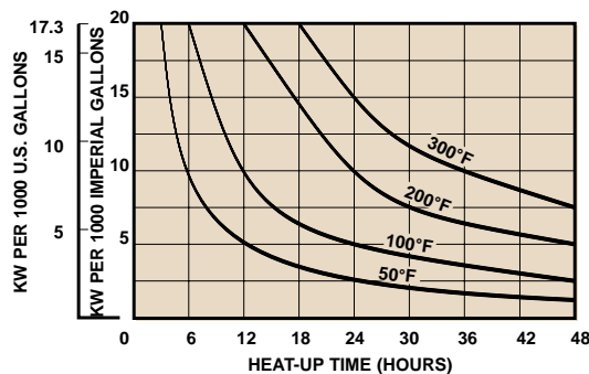
FIG. 4 - TANK CAPACITY vs. HEAT-UP TIME FOR ASPHALT
