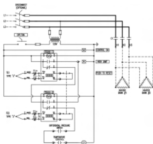
Package #1 - Basic Unit (ON/OFF Control)
