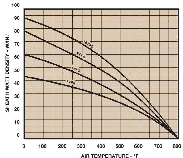
FIG. 1 - WATT DENSITY VS. AIR TEMPERATURE FOR 797°F (425°C) FIN TEMPERATURE
