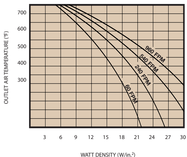
FIG. 3 - FINNED STRIP HEATER OUTLET AIR TEMPERATURE vs. WATT DENSITY FOR 700 - 750°F SHEATH OPERATING TEMPERATURE
