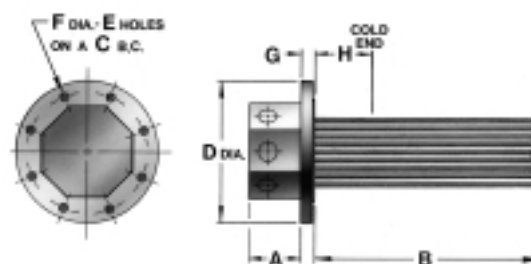
HEATER DIMENSIONS IN INCHES
