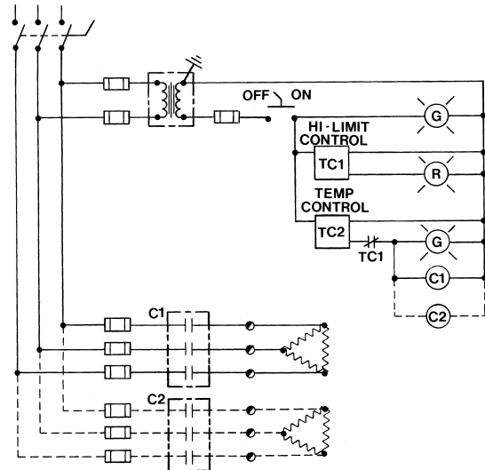
FIG. 5 - TYPICAL CONTROL SYSTEM
