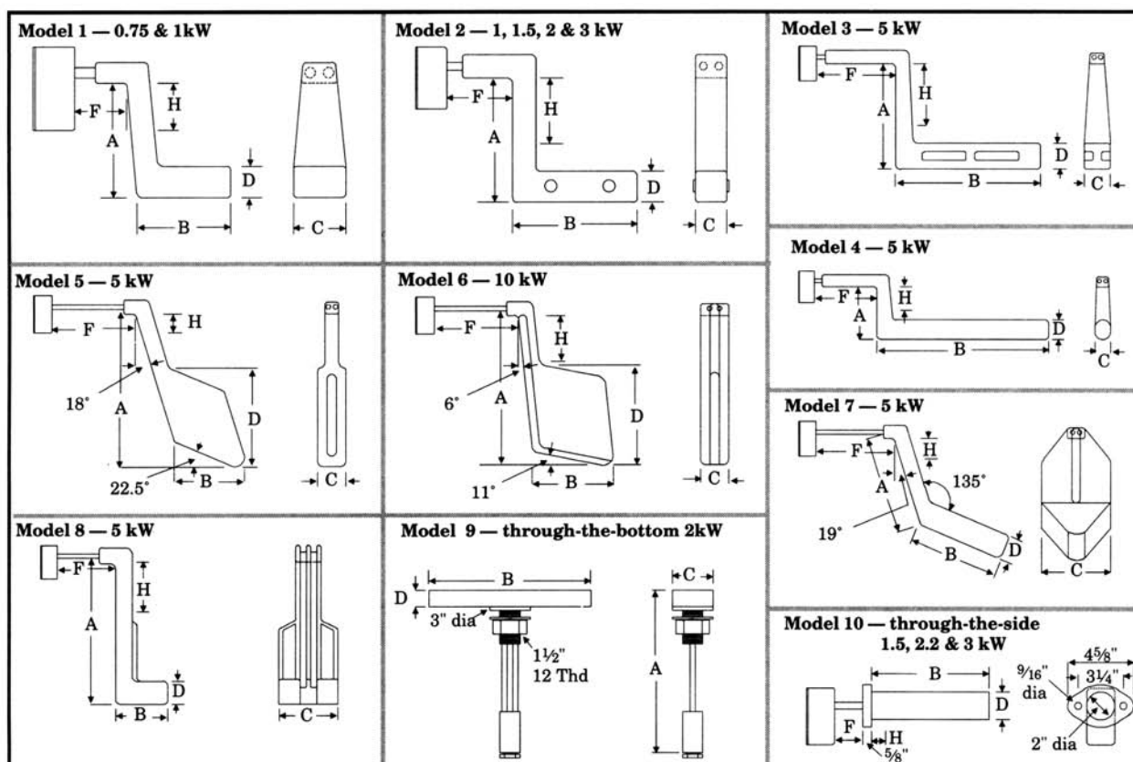
FIG. 1 - TYPE MC CAST-IN HEATERS
