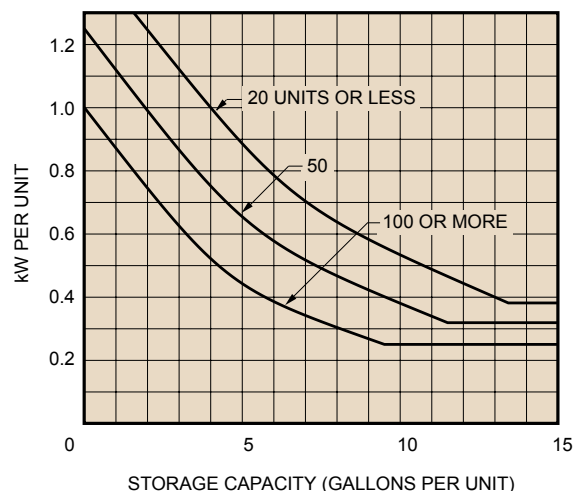
FIG. 2 - MOTELS
