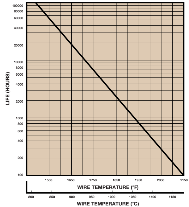
FIG. 1 - Life vs. Coil Temperature (Typical)
