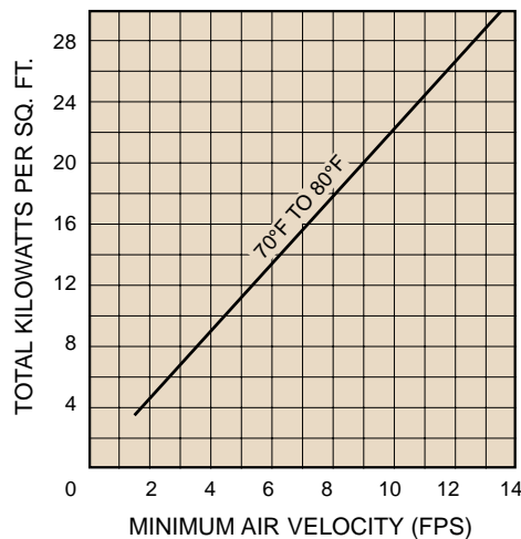
FIG. 6 - AIR VELOCITY REQUIREMENTS
