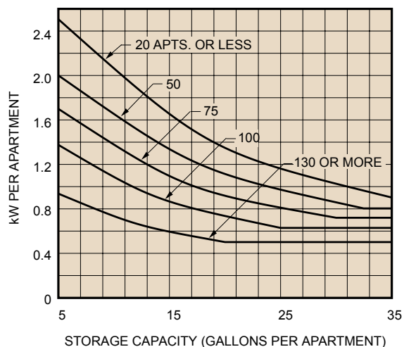
FIG. 3 - APARTMENT BUILDINGS
