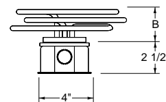
FIG. 3 - Three Element Unit
