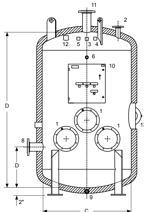
FIG. 6 - TYPE VC CALORIFIER
