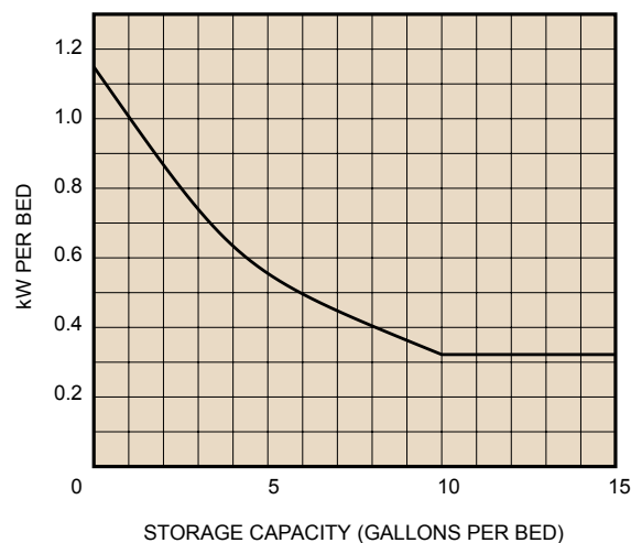
FIG. 4 - NURSING HOMES
