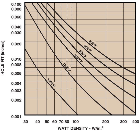
FIG. 2 - ALLOWABLE WATT DENSITY VS. FIT TOLERANCE AND WORK TEMPERATURE
