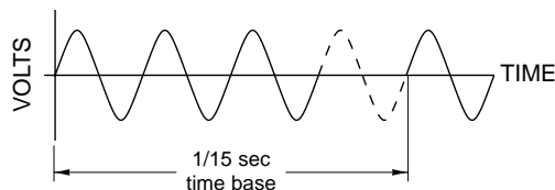
FIGURE 3 - Variable time base at 75% output
