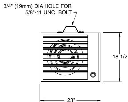
FIGURE 2 - HORIZONTAL AIR FLOW CEILING MOUNT
