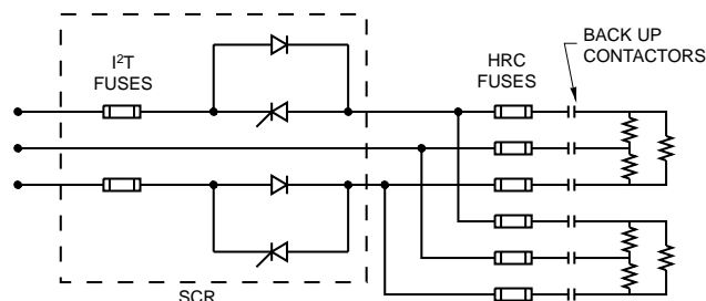
FIGURE 4 - SCR with back-up contactors
