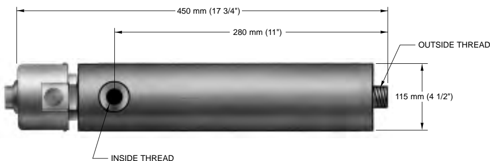
FIG. 1 - UNIT WITH BUILT-IN THERMOSTAT SHOWN
