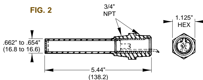
MOD 8A Moisture Resistant Seal On Adjusting Sleeve
