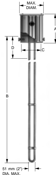
FIG. 1 - TYPE MXG HEATER
