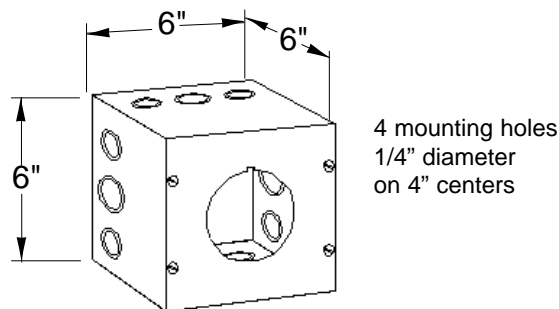
FIG. 2 Surface mounting enclosure
