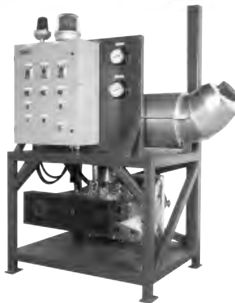
CRUCIBLE PREHEATER 600V 22KW 400 SCFM 250°C OUTLET
