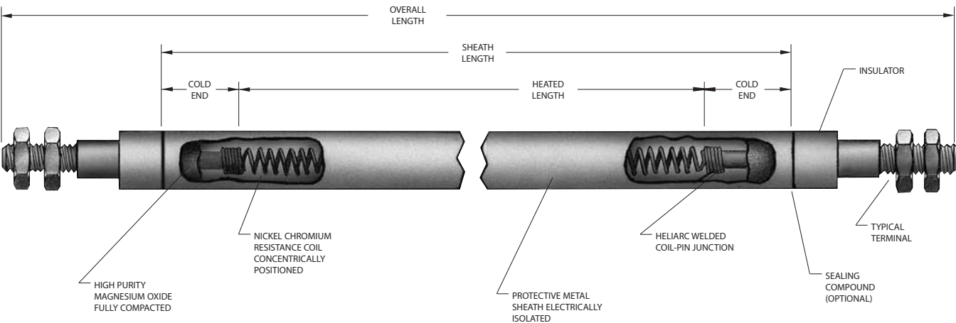
FIG. 1 - Tubular Element Features and Components
