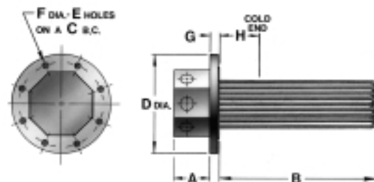
HEATER DIMENSIONS IN INCHES
