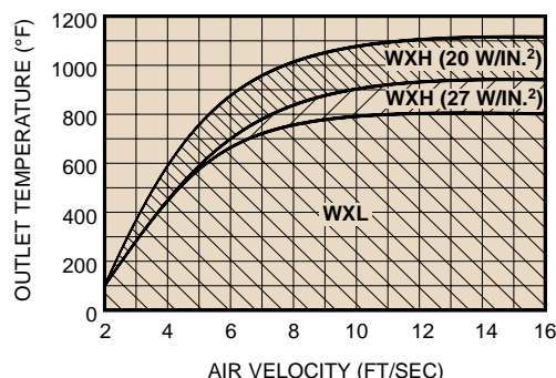
FIG. 1 - HEATER SELECTION
