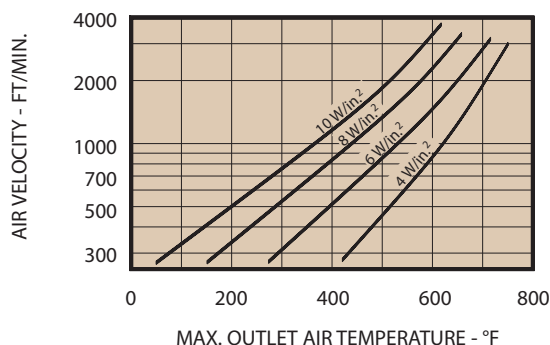
FIG. 4 - VELOCITY VS. AIR TEMPERATURE FOR 800°F (425°C) FIN TEMPERATURE
