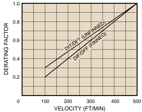
FIG.7 - DERATING FACTORS
