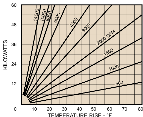
FIG. 3 - RECOMMENDED KILOWATTS
