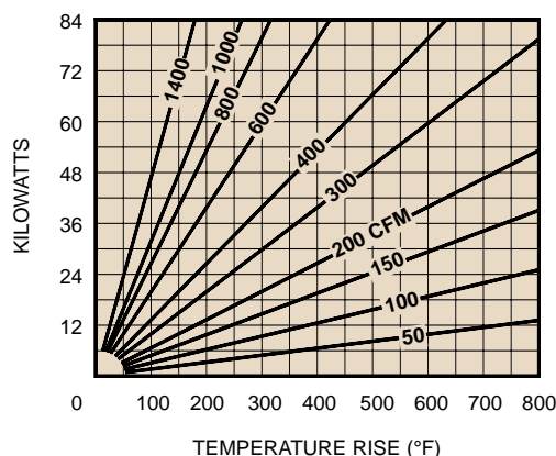
FIG. 2 - RECOMMENDED KILOWATTS
