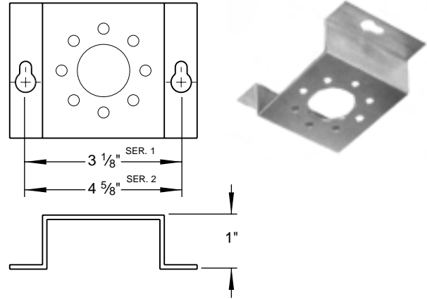
FIG. 1 - The x-Max ® universal mounting bracket
