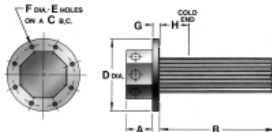
HEATER DIMENSIONS IN INCHES
