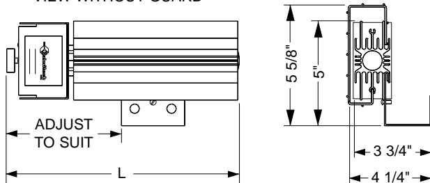
VIEW WITHOUT GUARD
