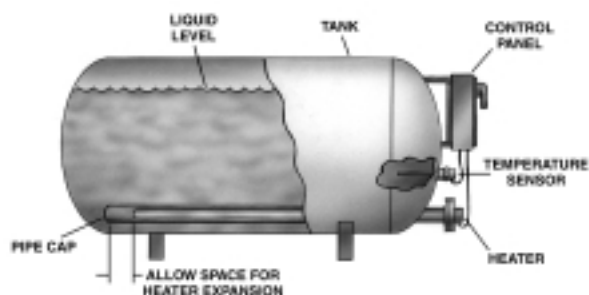
FIG. 1 - Typical application of pipe-insert immersion heater for viscous fluids
